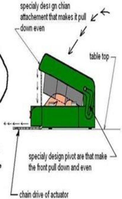
Enlarge View of the chicken cutter shown how blades work to adjust of bird and to min. motor requirements so this appliance works like a chainsaw never cutting thru more than one bone at a time
